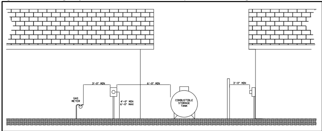
Figure 13. Metering Profile Elevation and Clearance Requirements Drawing
